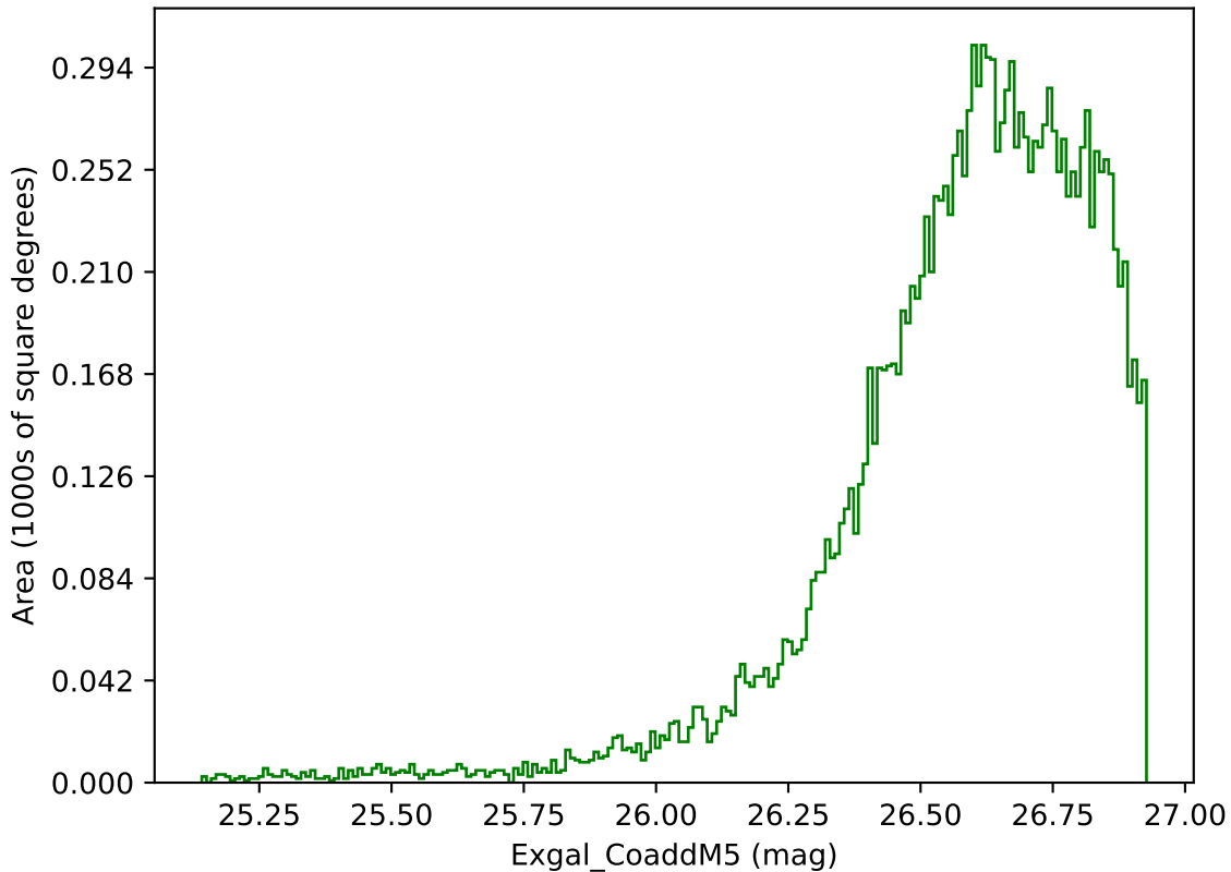
ddf_acor_sf20_lsf30_lsr50_v3.4_10yrs WFD g band: Exgal_CoaddM5
