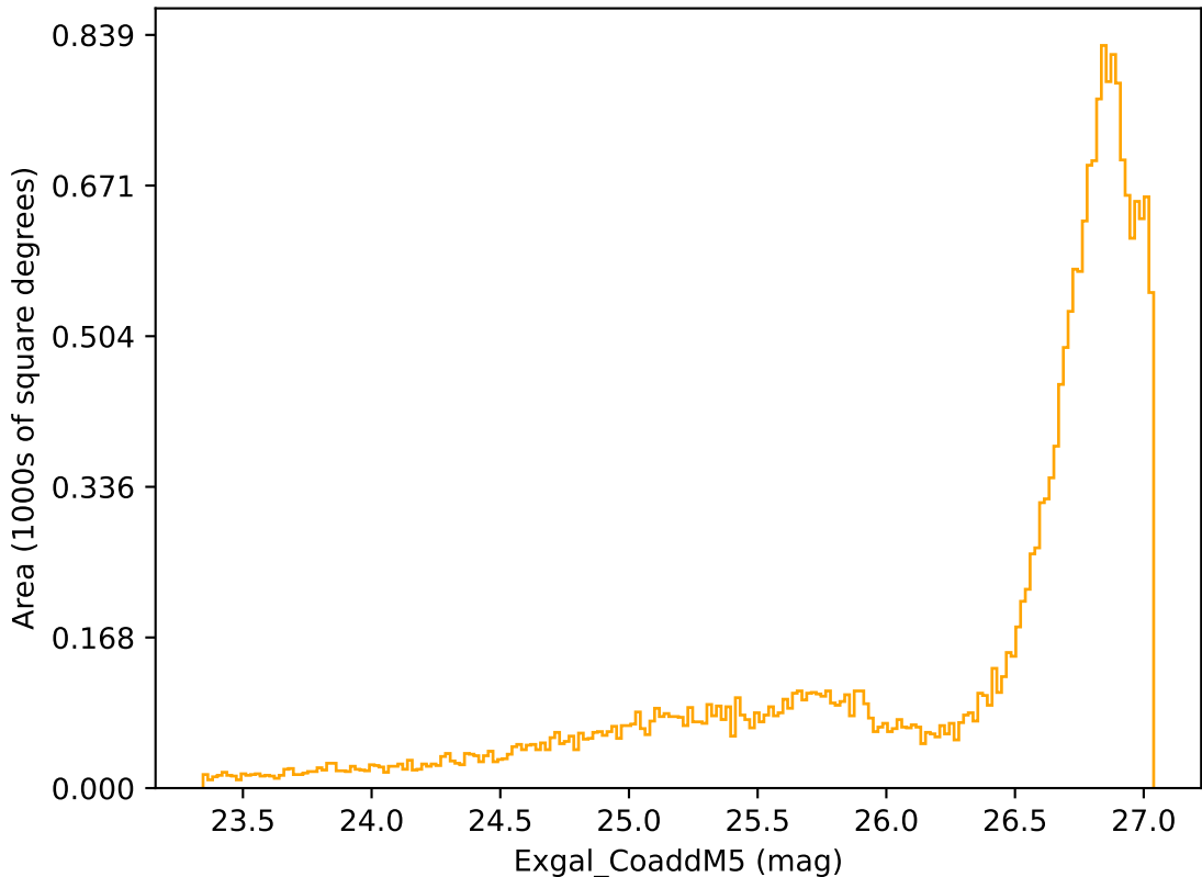
ddf_acor_sf20_lsf30_lsr50_v3.4_10yrs All sky r band: Exgal_CoaddM5
