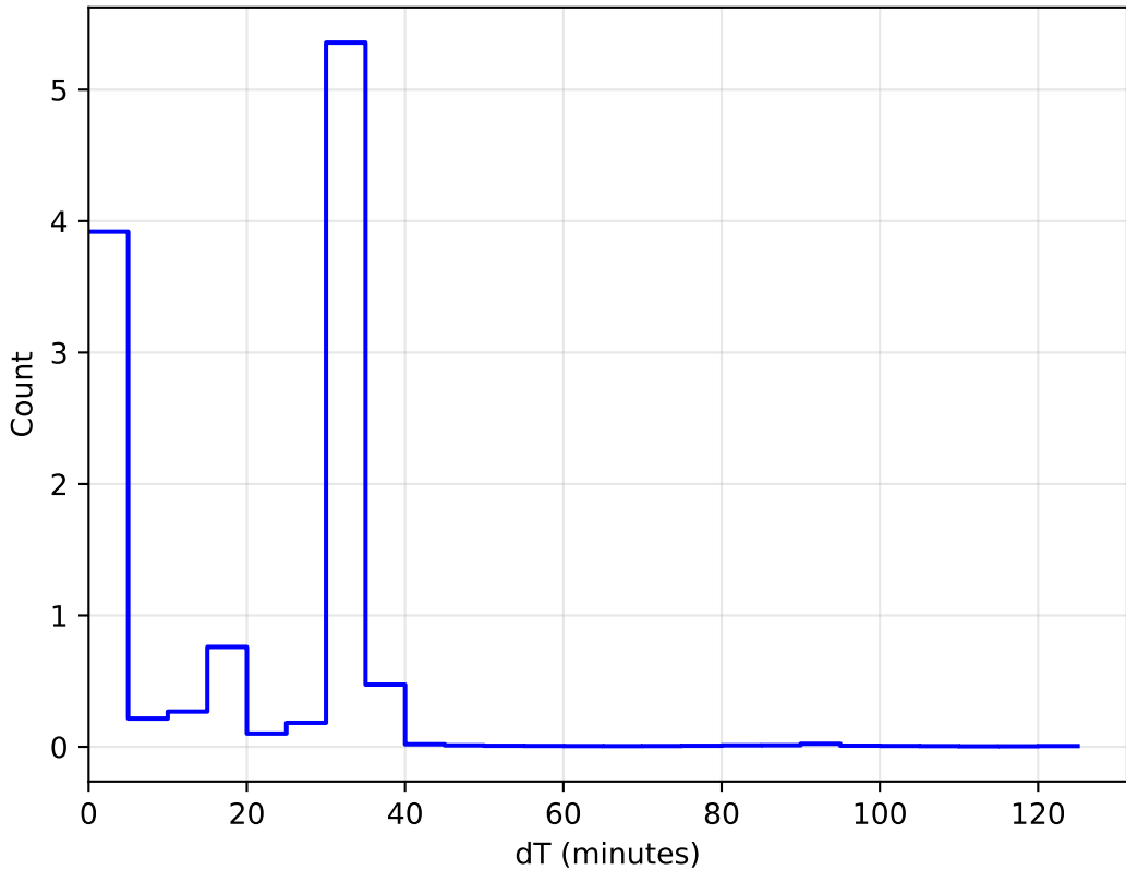
ddf_acor_sf20_lsf30_lsr50_v3.4_10yrs WFD: DeltaT Histogram 1e6
