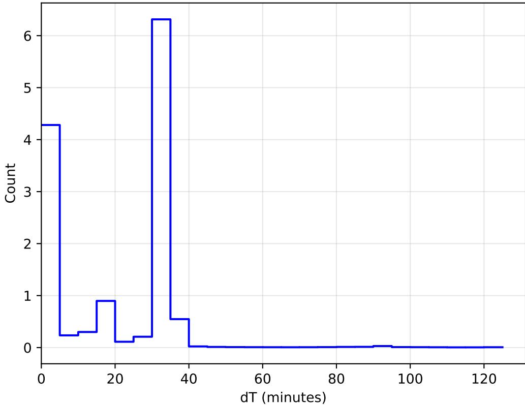
ddf_acor_sf20_lsf30_lsr50_v3.4_10yrs All sky: DeltaT Histogram
