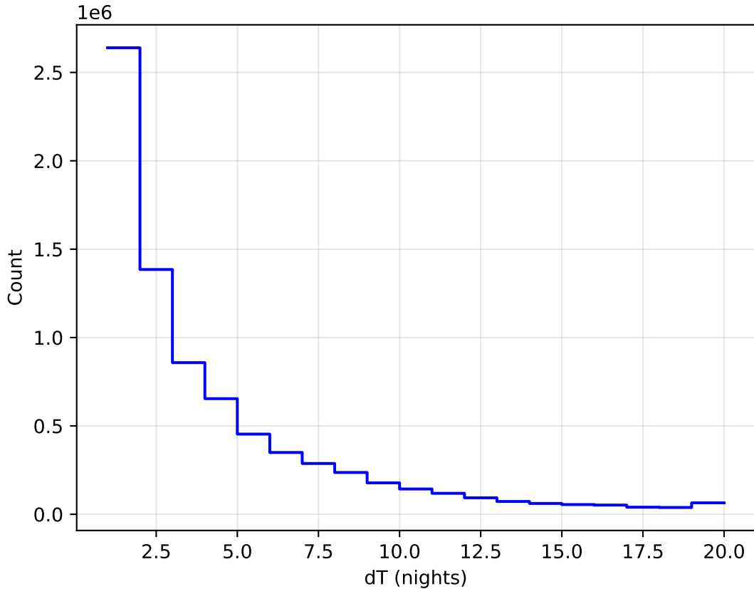
ddf_acor_sf20_lsf30_lsr50_v3.4_10yrs WFD all bands: DeltaNight Histogram
