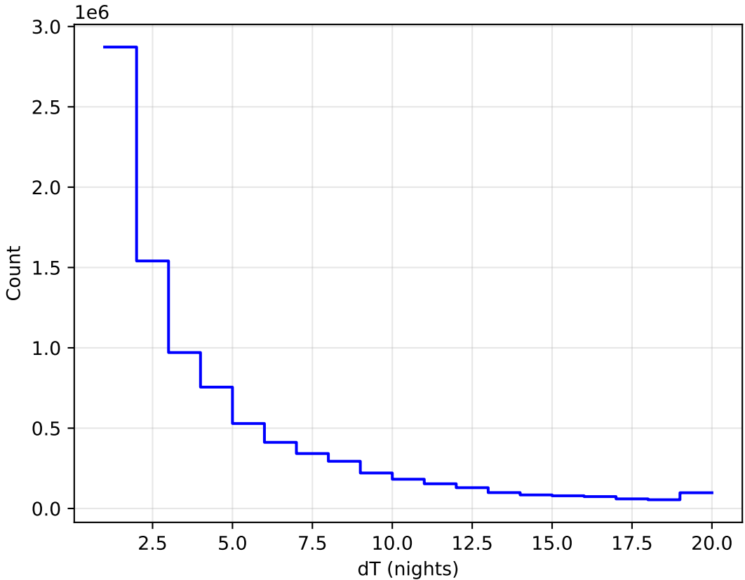
ddf_acor_sf20_lsf30_lsr50_v3.4_10yrs All sky all bands: DeltaNight Histogram
