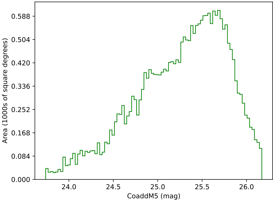
ddf_acor_sf20_lsf30_lsr50_v3.4_10yrs Yr 3-4 g band: CoaddM5
