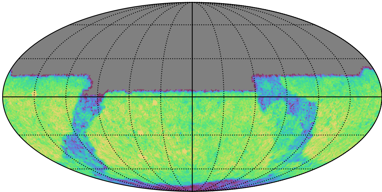
ddf_acor_sf20_lsf30_lsr50_v3.4_10yrs Yr 1 y band: CoaddM5
