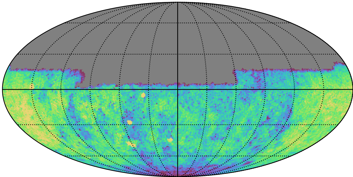
ddf_acor_sf20_lsf30_lsr50_v3.4_10yrs Yr 1 u band: CoaddM5
