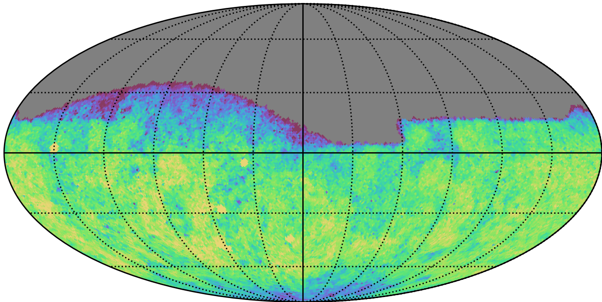
ddf_acor_sf20_lsf30_lsr50_v3.4_10yrs Yr 1 g band: CoaddM5
