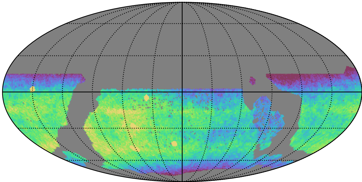
ddf_acor_sf20_lsf30_lsr50_v3.4_10yrs WFD z band: CoaddM5
