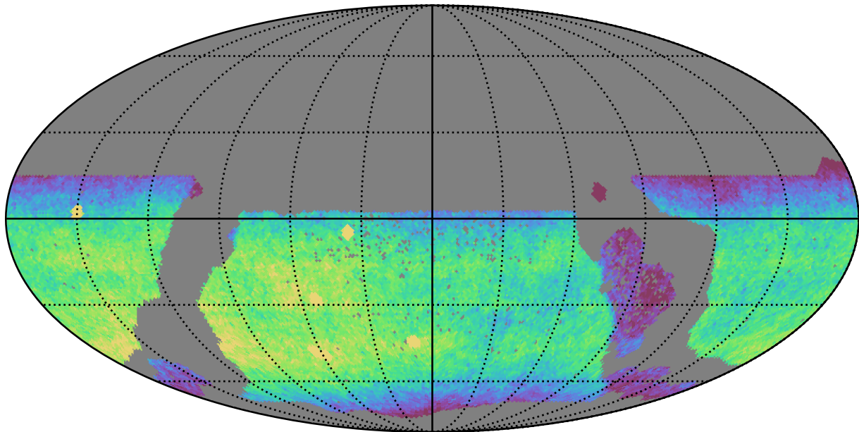
ddf_acor_sf20_lsf30_lsr50_v3.4_10yrs WFD y band: CoaddM5
