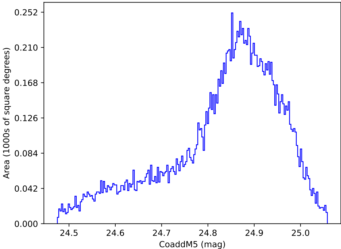
ddf_acor_sf20_lsf30_lsr50_v3.4_10yrs WFD y band: CoaddM5
