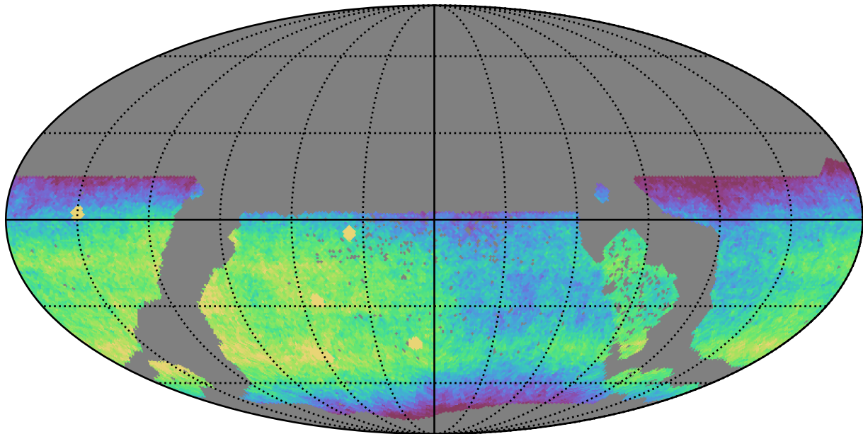
ddf_acor_sf20_lsf30_lsr50_v3.4_10yrs WFD r band: CoaddM5
