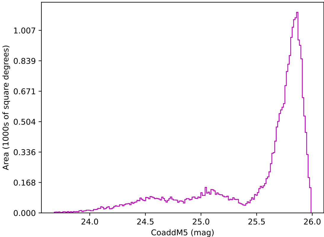
ddf_acor_sf20_lsf30_lsr50_v3.4_10yrs All sky z band: CoaddM5
