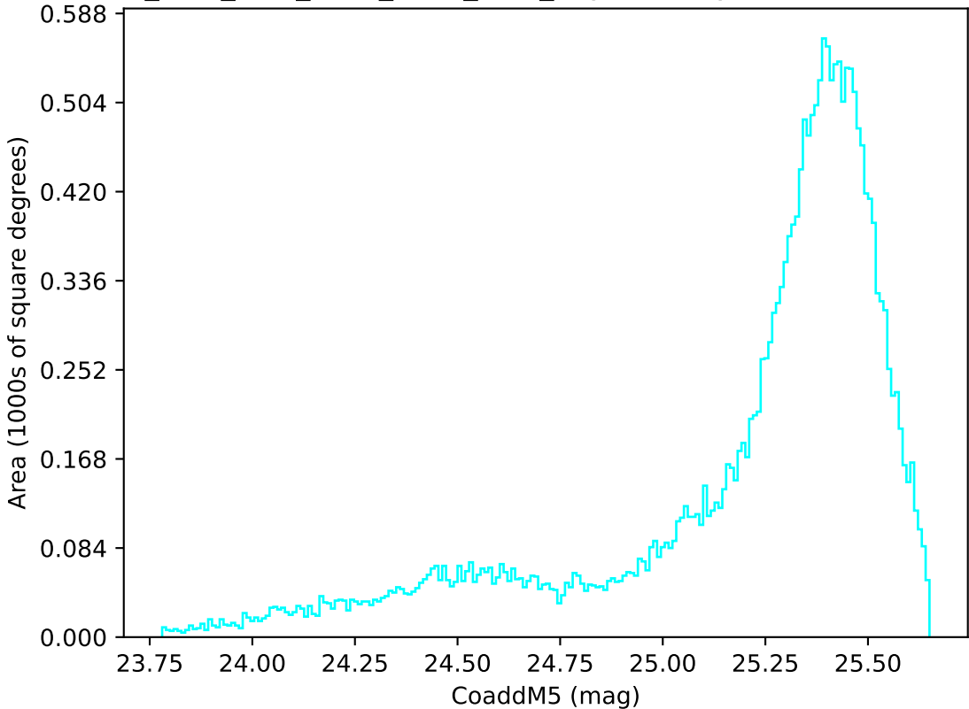
ddf_acor_sf20_lsf30_lsr50_v3.4_10yrs All sky u band: CoaddM5
