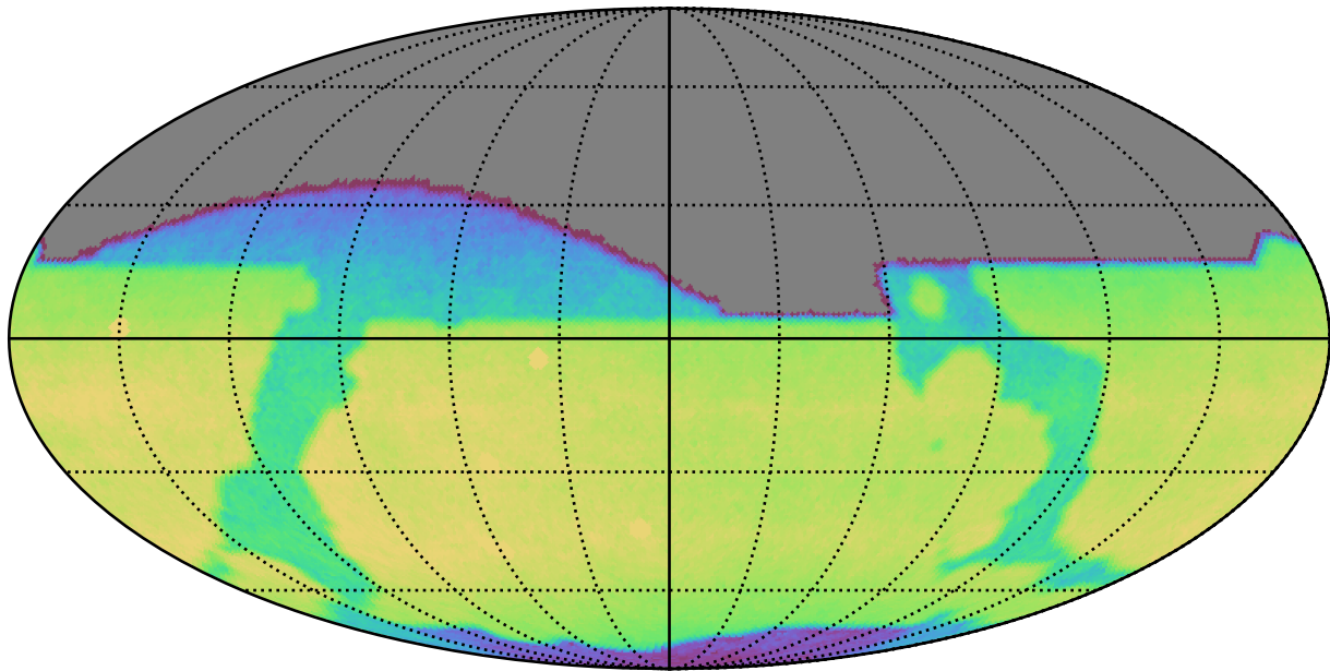
ddf_acor_sf20_lsf30_lsr50_v3.4_10yrs All sky i band: CoaddM5
