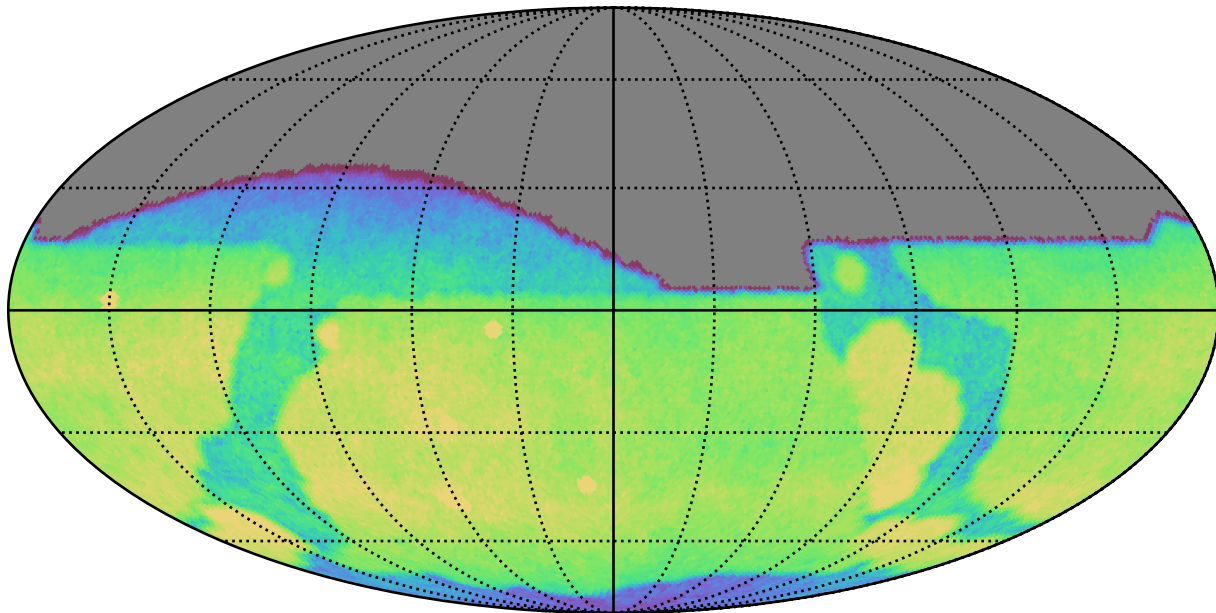
ddf_acor_sf20_lsf30_lsr50_v3.4_10yrs All sky g band: CoaddM5
