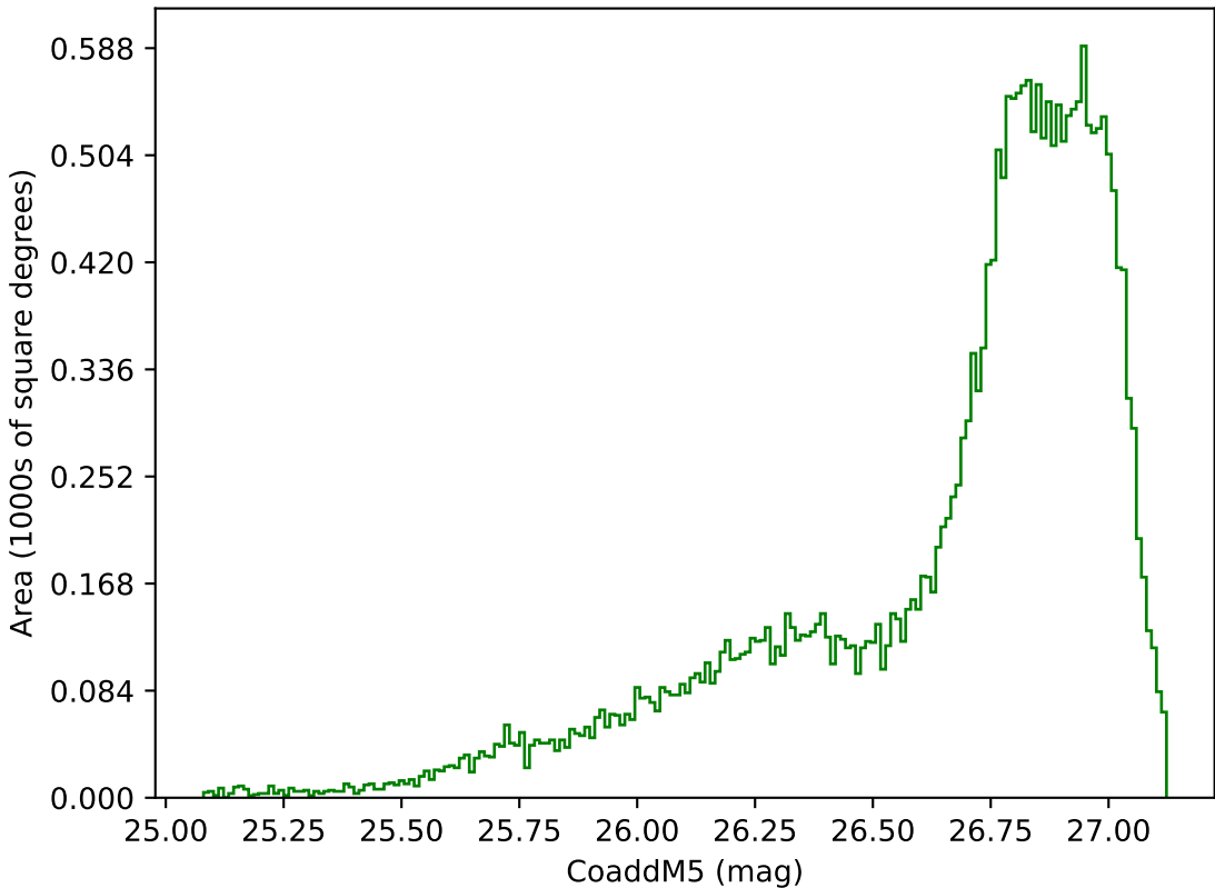
ddf_acor_sf20_lsf30_lsr50_v3.4_10yrs All sky g band: CoaddM5
