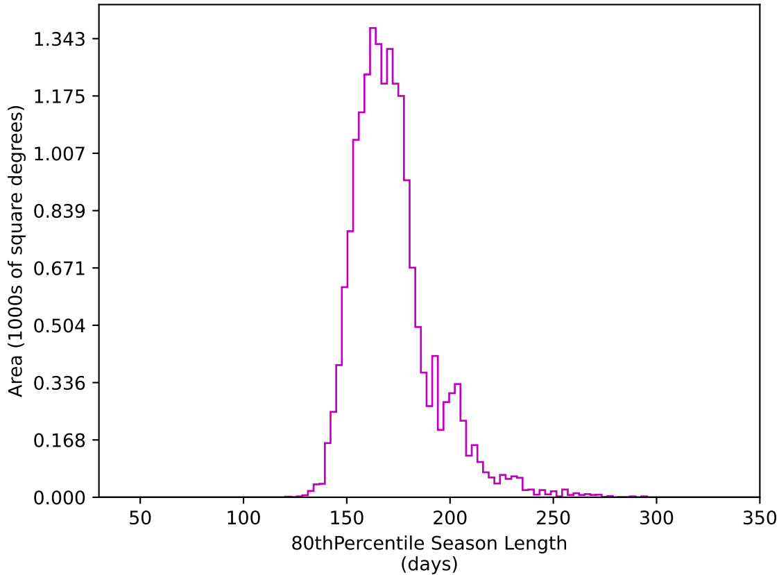
ddf_acor_sf20_lsf30_lsr50_v3.4_10yrs WFD z band: 80thPercentile Season Length
