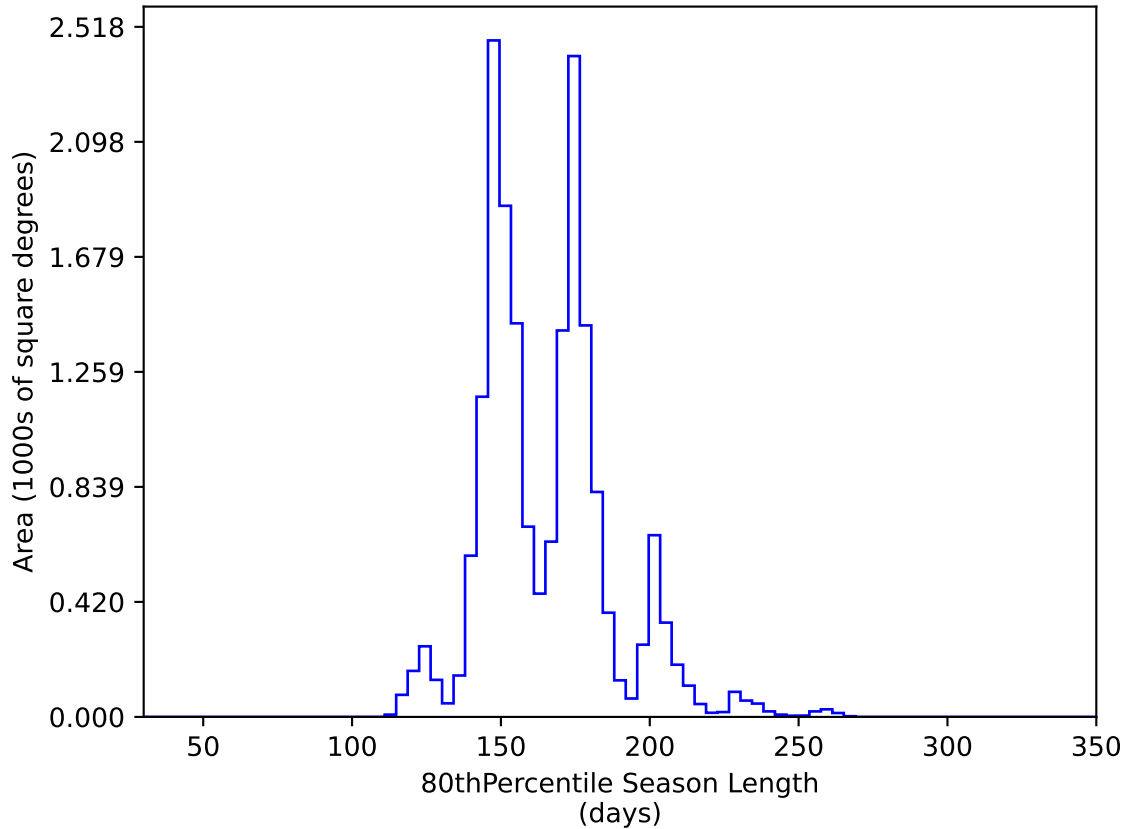
ddf_acor_sf20_lsf30_lsr50_v3.4_10yrs WFD y band: 80thPercentile Season Length
