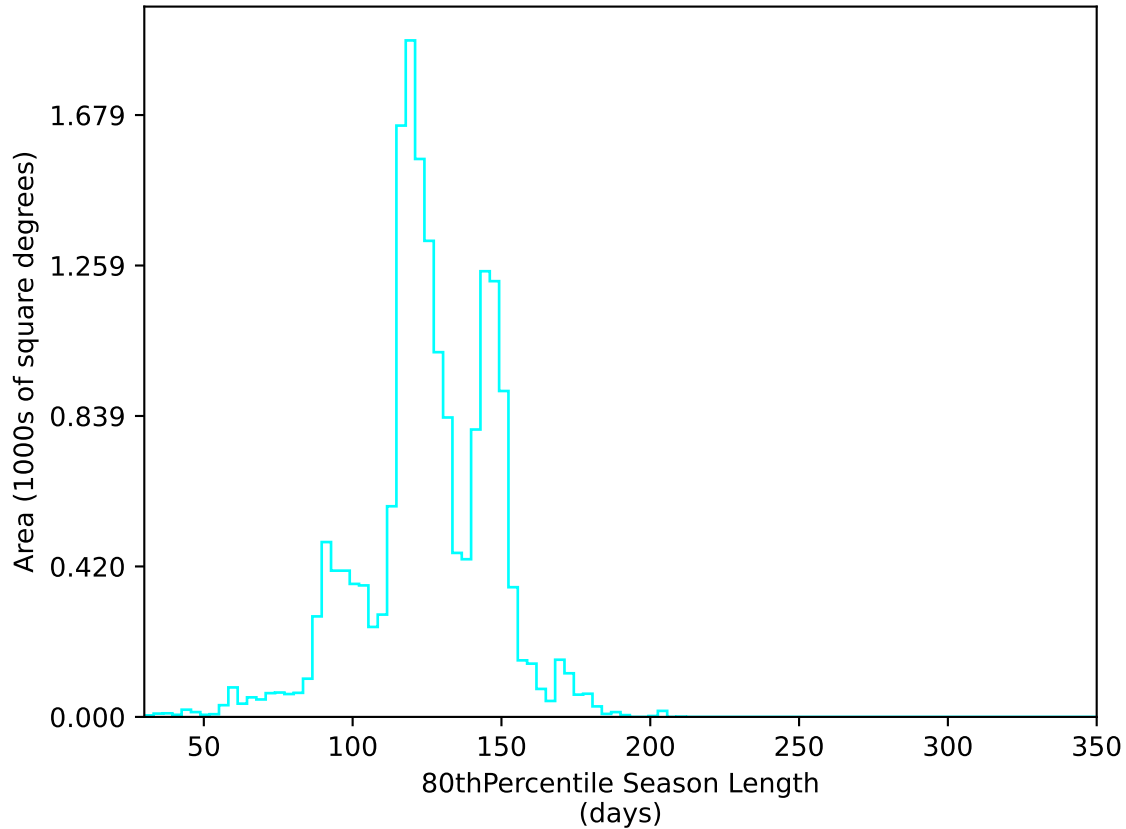
ddf_acor_sf20_lsf30_lsr50_v3.4_10yrs WFD u band: 80thPercentile Season Length
