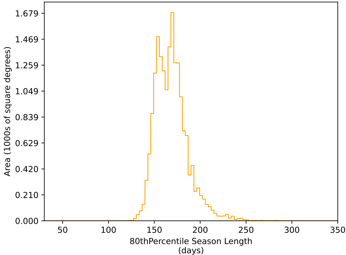
ddf_acor_sf20_lsf30_lsr50_v3.4_10yrs WFD r band: 80thPercentile Season Length
