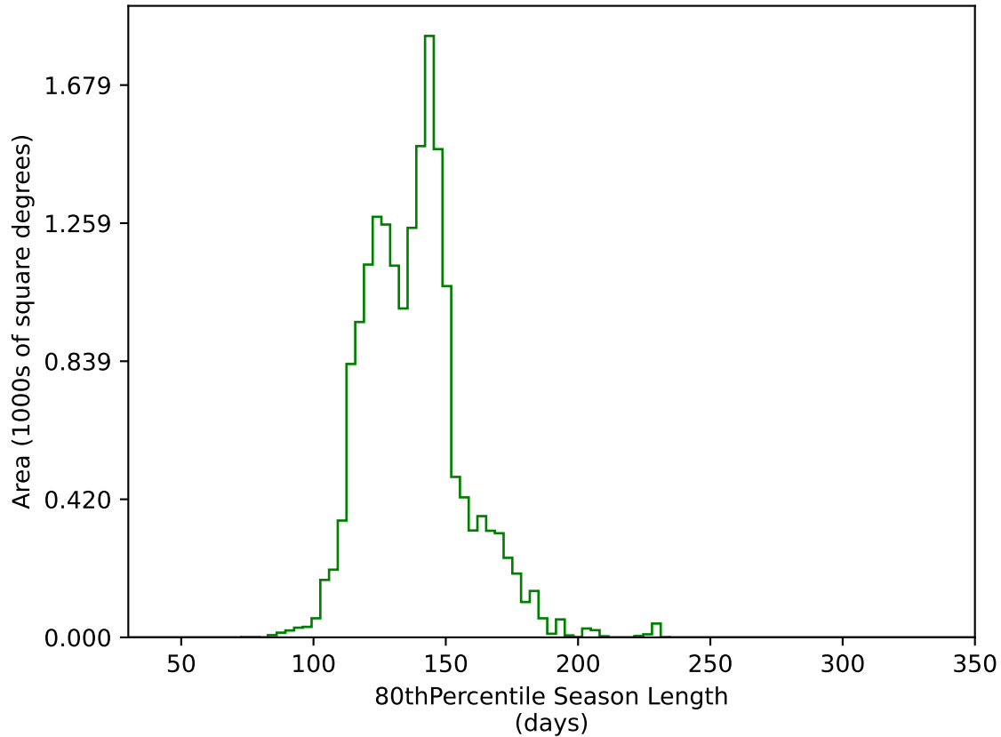
ddf_acor_sf20_lsf30_lsr50_v3.4_10yrs WFD g band: 80thPercentile Season Length
