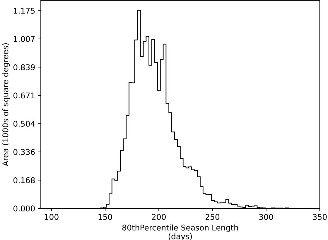
ddf_acor_sf20_lsf30_lsr50_v3.4_10yrs WFD all bands: 80thPercentile Season Length
