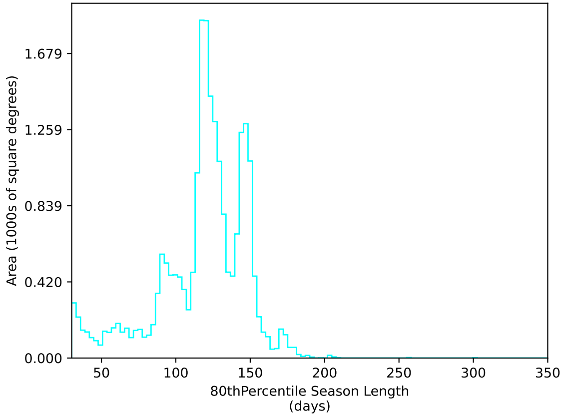
ddf_acor_sf20_lsf30_lsr50_v3.4_10yrs All sky u band: 80thPercentile Season Length
