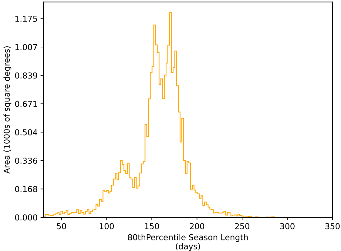
ddf_acor_sf20_lsf30_lsr50_v3.4_10yrs All sky r band: 80thPercentile Season Length
