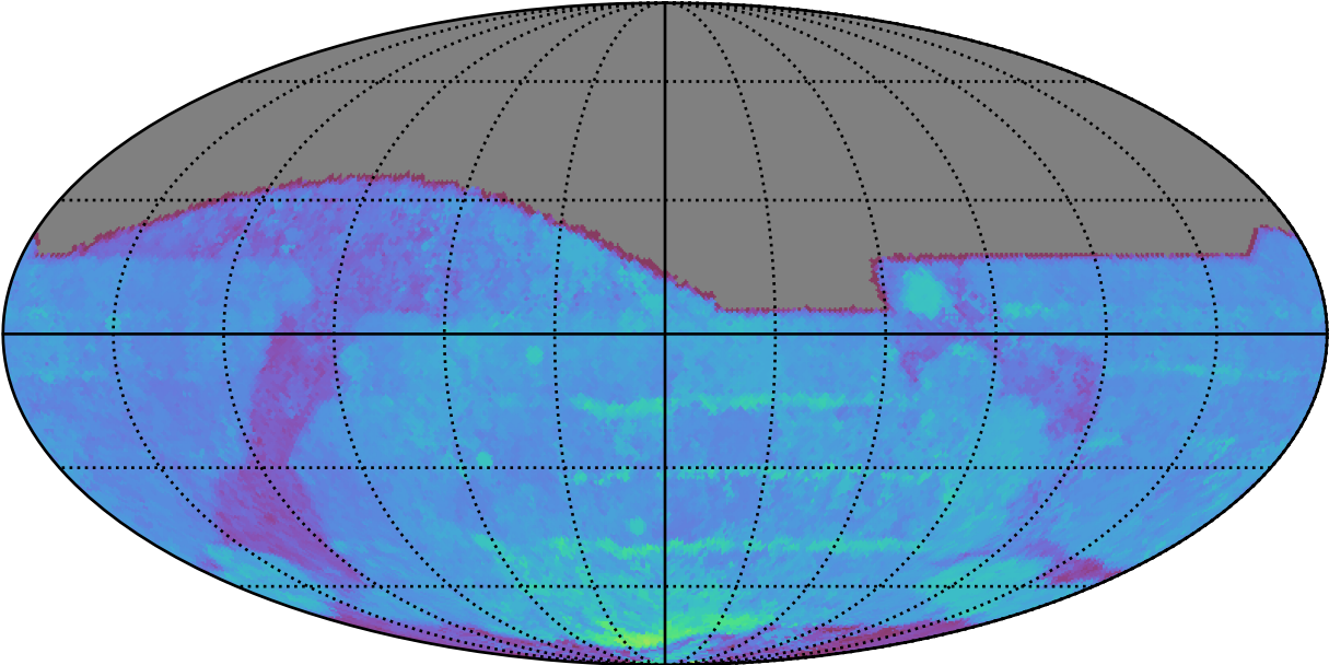
ddf_acor_sf20_lsf30_lsr50_v3.4_10yrs All sky i band: 80thPercentile Season Length
