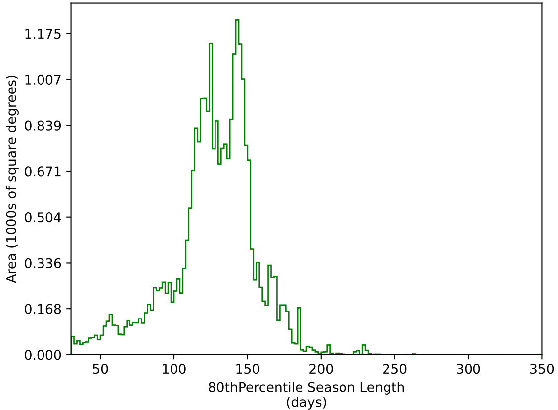
ddf_acor_sf20_lsf30_lsr50_v3.4_10yrs All sky g band: 80thPercentile Season Length
