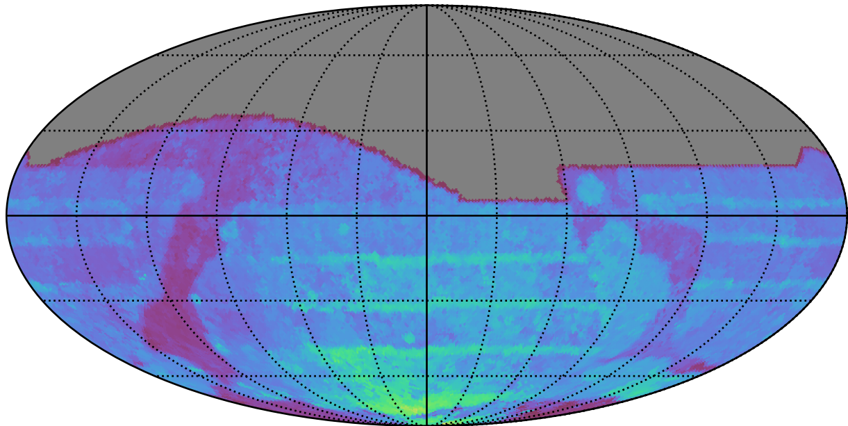
ddf_acor_sf20_lsf30_lsr50_v3.4_10yrs All sky all bands: 80thPercentile Season Length
