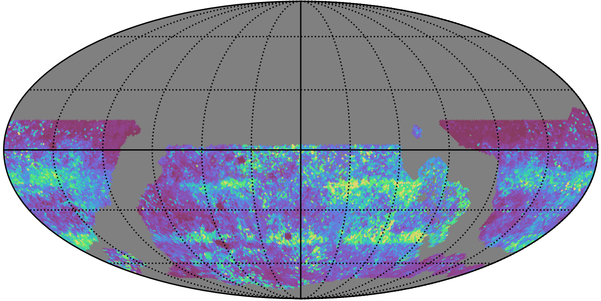
ddf_acor_sf20_lsf30_lsr50_v3.4_10yrs WFD zy bands: 75th Percentile Intranight Timespan
