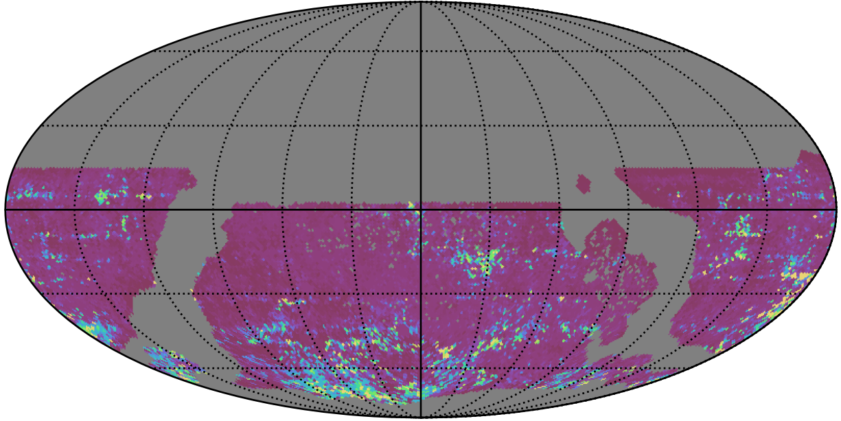
ddf_acor_sf20_lsf30_lsr50_v3.4_10yrs WFD z band: 75th Percentile Intranight Timespan
