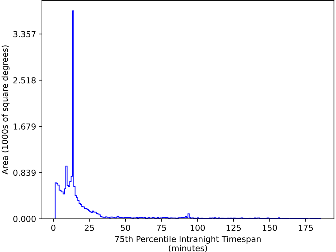
ddf_acor_sf20_lsf30_lsr50_v3.4_10yrs WFD z band: 75th Percentile Intranight Timespan
