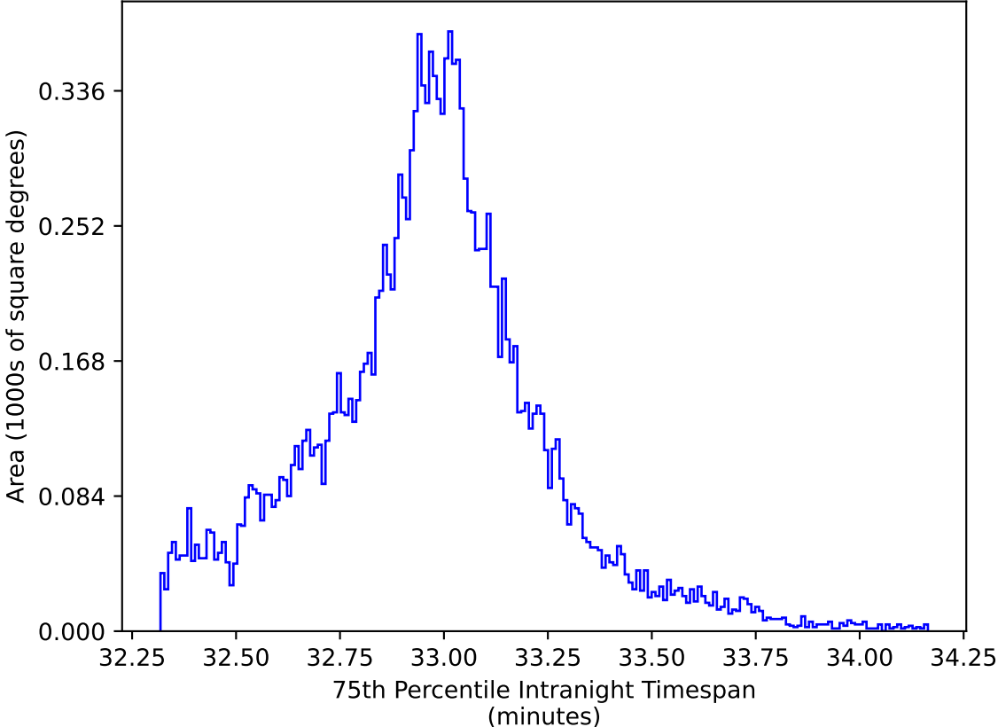
ddf_acor_sf20_lsf30_lsr50_v3.4_10yrs WFD y band: 75th Percentile Intranight Timespan
