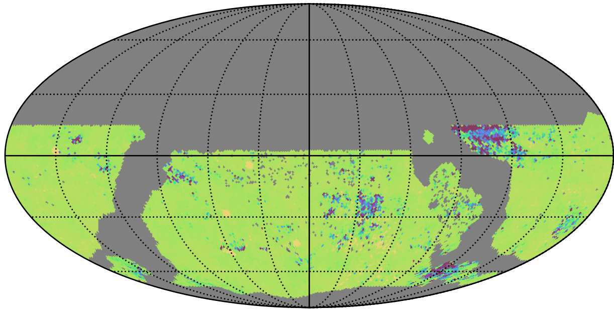
ddf_acor_sf20_lsf30_lsr50_v3.4_10yrs WFD ug bands: 75th Percentile Intranight Timespan
