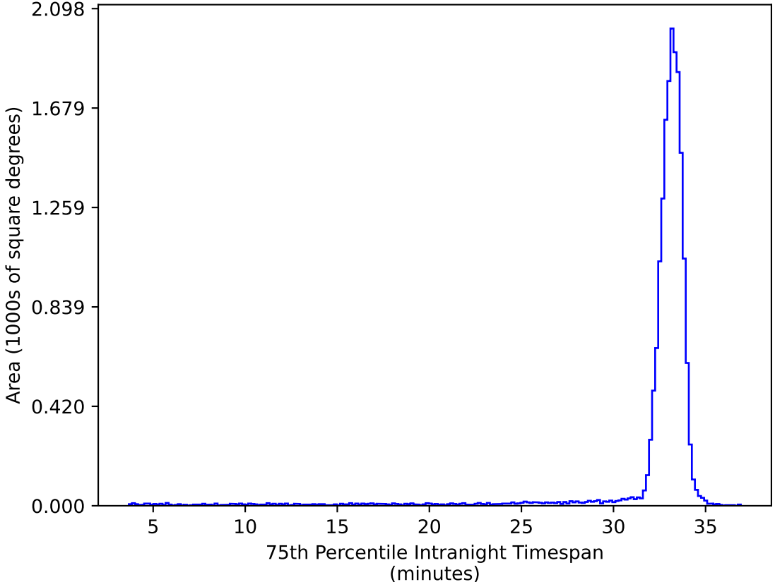
ddf_acor_sf20_lsf30_lsr50_v3.4_10yrs WFD ug bands: 75th Percentile Intranight Timespan
