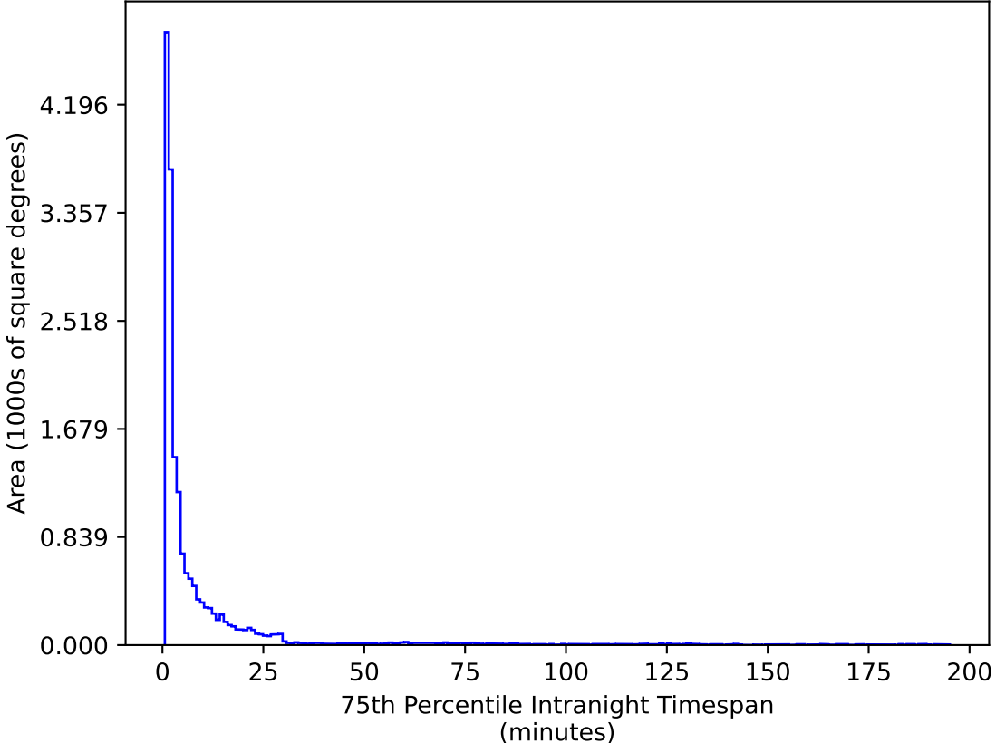
ddf_acor_sf20_lsf30_lsr50_v3.4_10yrs WFD u band: 75th Percentile Intranight Timespan
