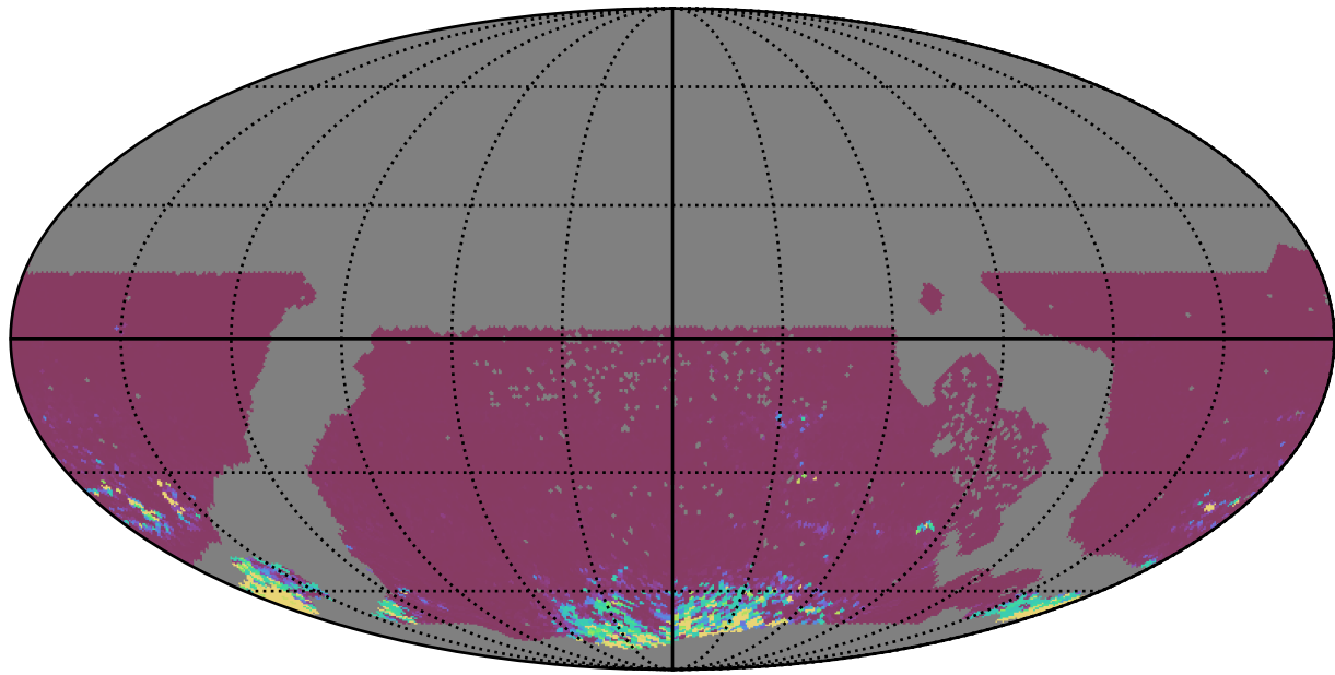
ddf_acor_sf20_lsf30_lsr50_v3.4_10yrs WFD ri bands: 75th Percentile Intranight Timespan
