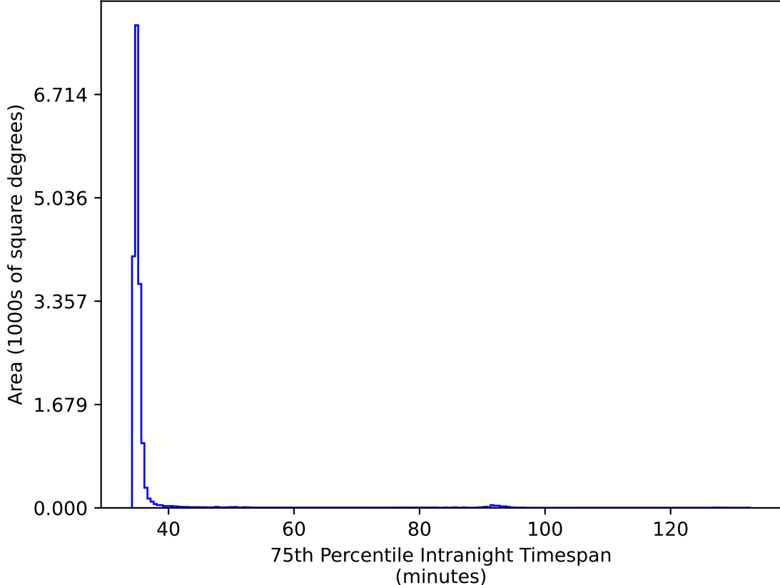
ddf_acor_sf20_lsf30_lsr50_v3.4_10yrs WFD ri bands: 75th Percentile Intranight Timespan
