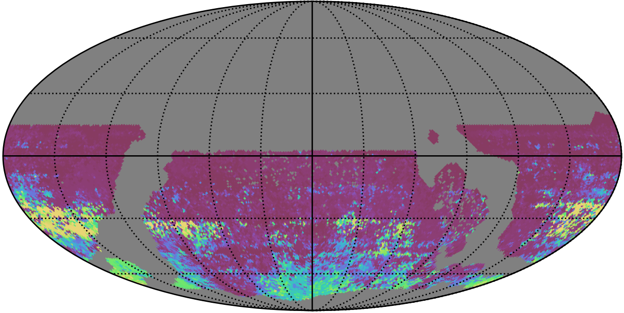
ddf_acor_sf20_lsf30_lsr50_v3.4_10yrs WFD r band: 75th Percentile Intranight Timespan
