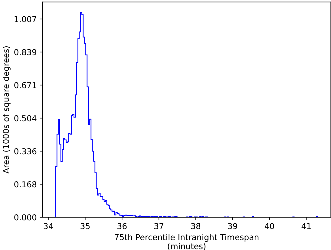
ddf_acor_sf20_lsf30_lsr50_v3.4_10yrs WFD iz bands: 75th Percentile Intranight Timespan
