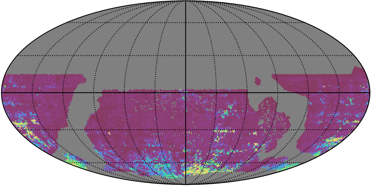
ddf_acor_sf20_lsf30_lsr50_v3.4_10yrs WFD i band: 75th Percentile Intranight Timespan
