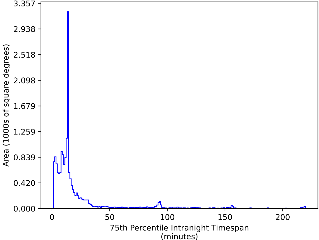
ddf_acor_sf20_ls30_isr50_v3.4_10yrs WFD i band: 75th Percentile Intranight Timespan
