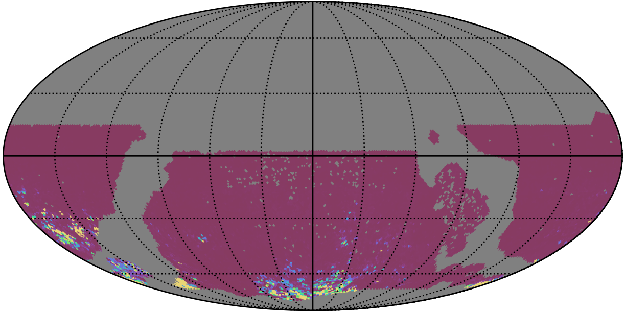
ddf_acor_sf20_lsf30_lsr50_v3.4_10yrs WFD gr bands: 75th Percentile Intranight Timespan
