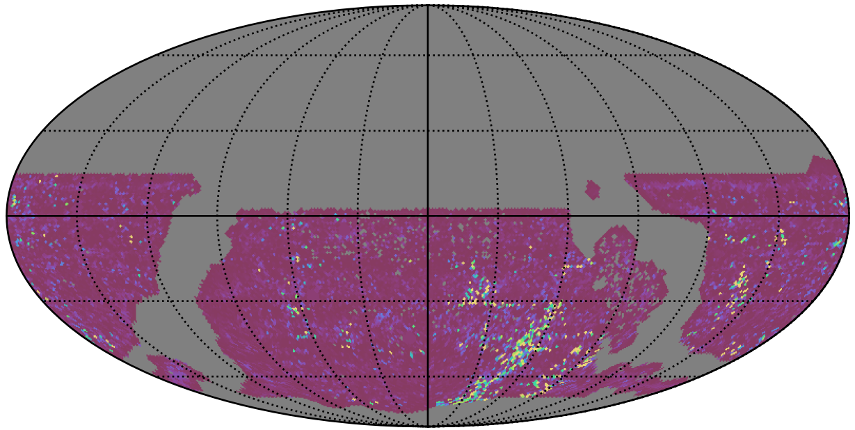
ddf_acor_sf20_lsf30_lsr50_v3.4_10yrs WFD g band: 75th Percentile Intranight Timespan
