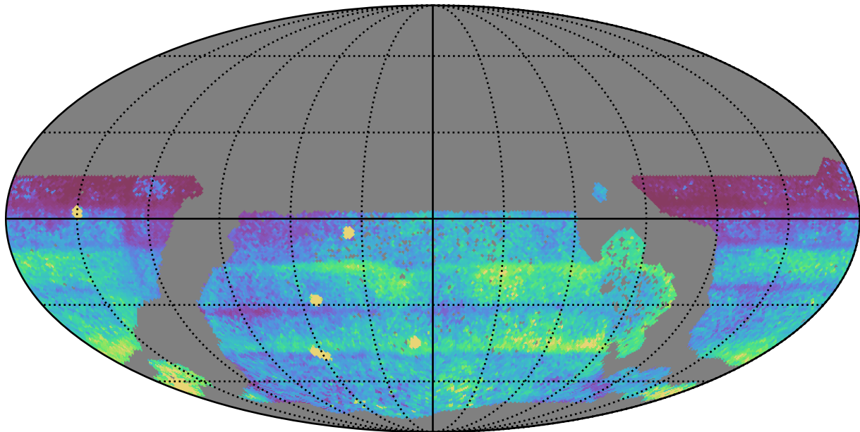
ddf_acor_sf20_lsf30_lsr50_v3.4_10yrs WFD all bands: 75th Percentile Intranight Timespan
