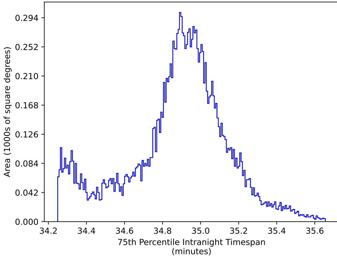
ddf_acor_sf20_lsf30_lsr50_v3.4_10yrs WFD all bands: 75th Percentile Intranight Timespan
