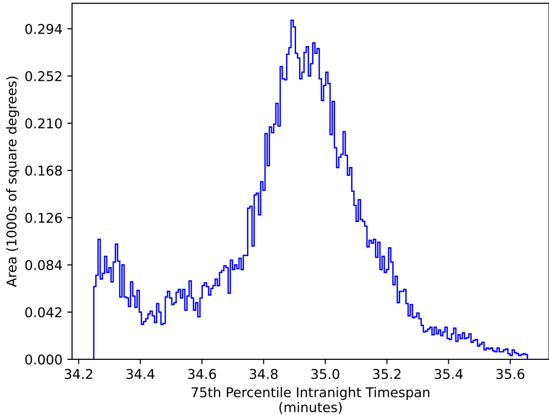
ddf_acor_sf20_ls30_lsr50_v3.4_10yrs WFD: 75th Percentile Intranight Timespan
