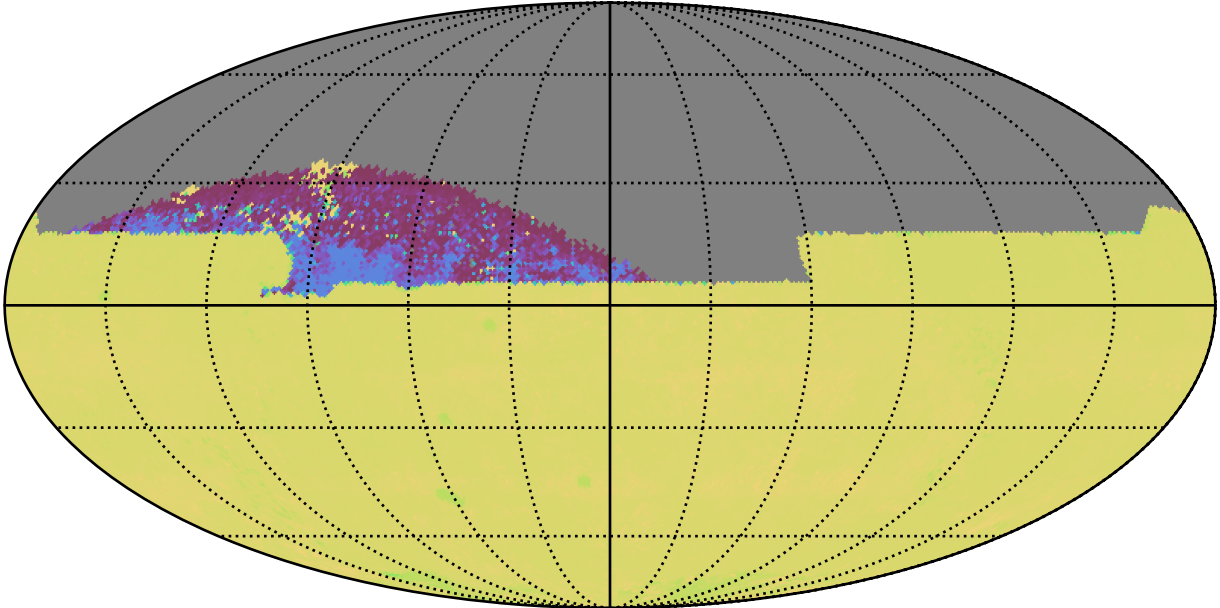
ddf_acor_sf20_lsf30_lsr50_v3.4_10yrs All sky zy bands: 75th Percentile Intranight Timespan
