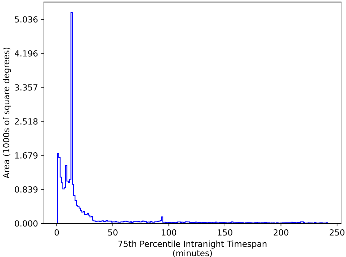
ddf_acor_sf20_lsf30_lsr50_v3.4_10yrs All sky z band: 75th Percentile Intranight Timespan
